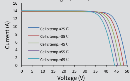
Current-Voltage (545W)
